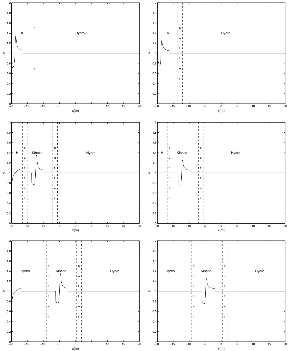
Fig. 5. Unsteady shock 1: Smoothness indicators for density (left) and velocity (right) at different times t = 0.002 (top), t = 0.02 (middle), t = 0.04 (bottom).
