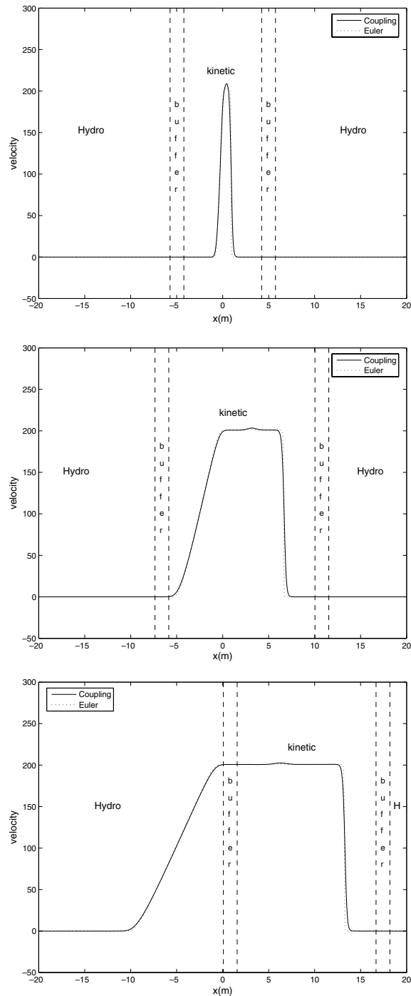
Fig. 13. Sod test 2: Velocity profile at different times t = 0.002 (top), t = 0.015 (middle), t = 0.03 (bottom). The solid line is the solution of the coupling model, the dotted line is that of the Euler system.
