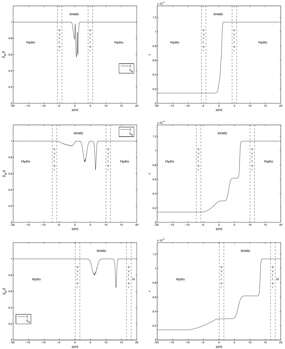
Fig. 14. Sod test 2: Equilibrium fraction profile (left), Knudsen number (right) at different times t = 0.002 (top), t = 0.015 (middle), t = 0.03 (bottom).
