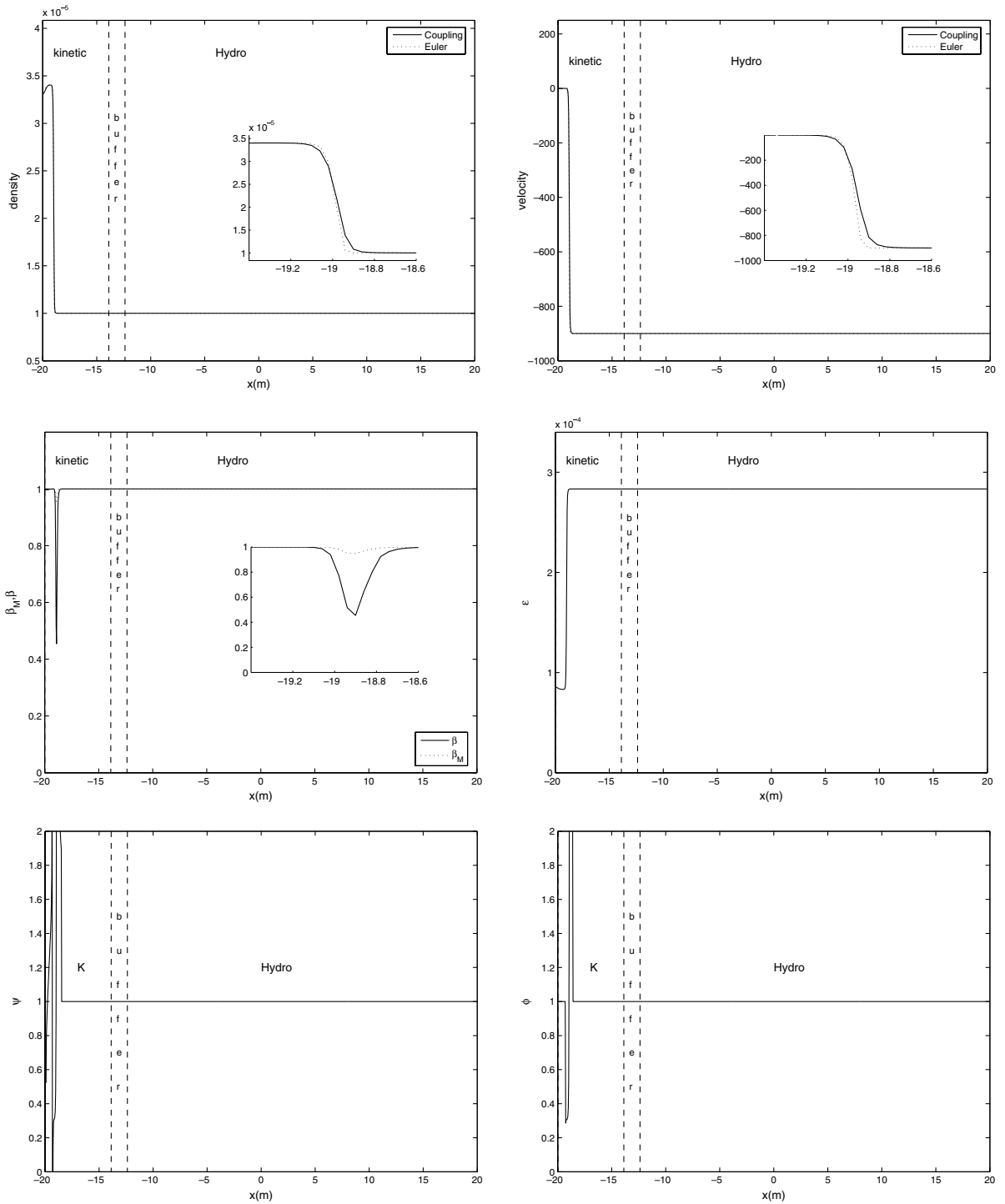
Fig. 6. Unsteady shock 2: Solution at t = 2 \times 10^{-3} . Density (top left), velocity (top right), equilibrium fraction (middle left), Knudsen number (middle right), density smoothness indicator (bottom left), velocity smoothness indicator (bottom right). The small panels are a magnification of the solution close to the shock.
