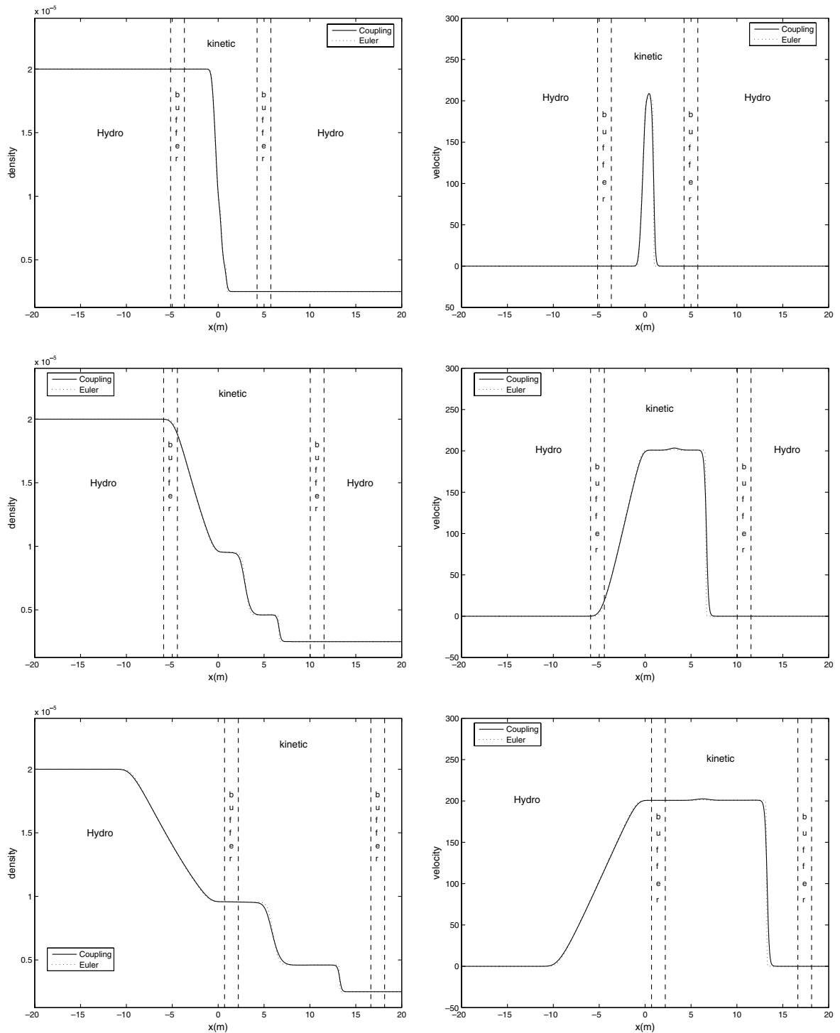
Fig. 16. Sod Test 3: Density (left), Velocity (right) profiles at different times t = 0.002 (top), t = 0.015 (middle), t = 0.03 (bottom). The solid line is the solution of the coupling model, the dotted line is that of the Euler system.
