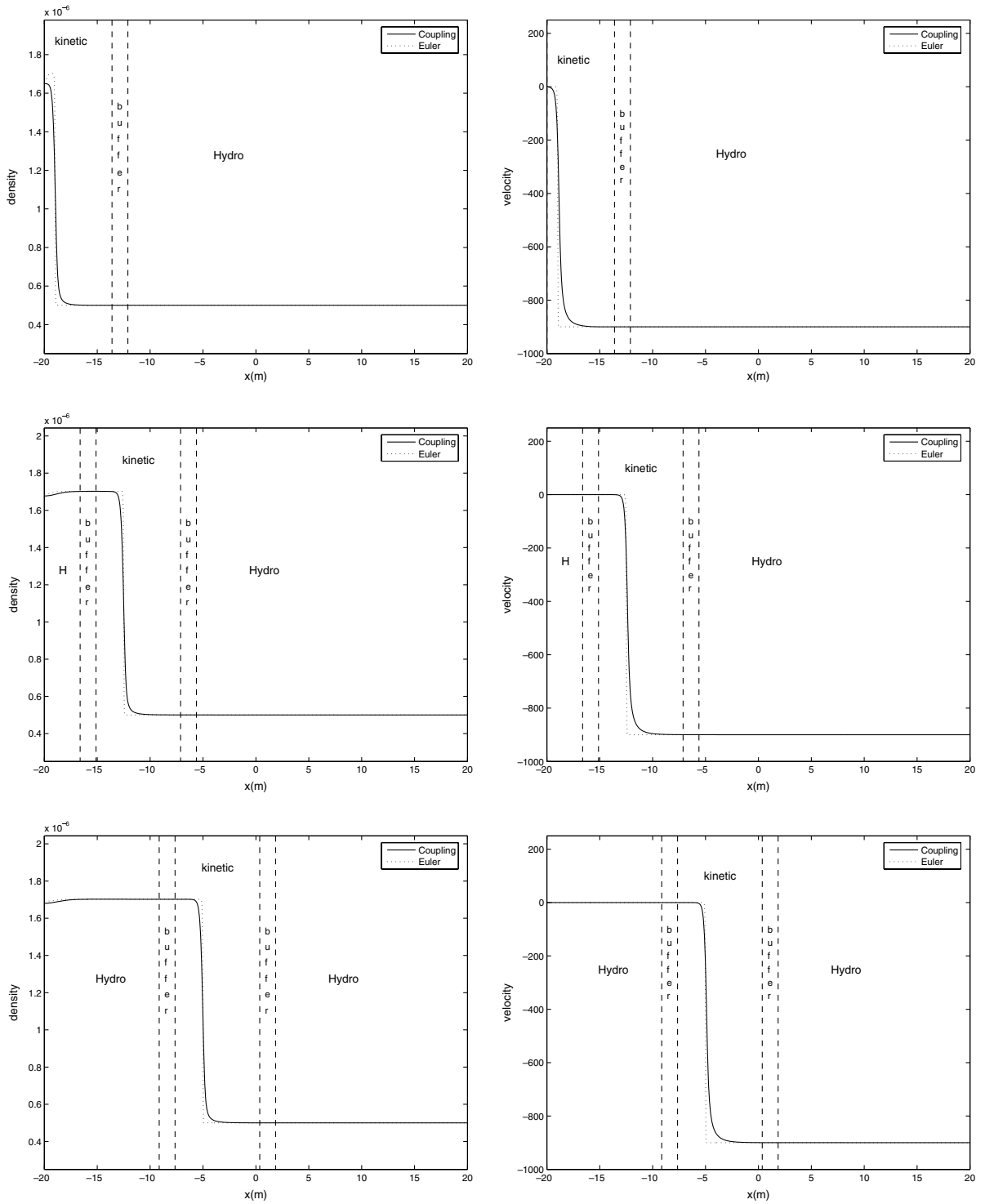
Fig. 17. Unsteady shock test: Density (left), Velocity (right) profiles at different times t = 0.002 (top), t = 0.02 (middle), t = 0.04 (bottom). The solid line is the solution of the coupling model, the dotted line is that of the Euler system.
