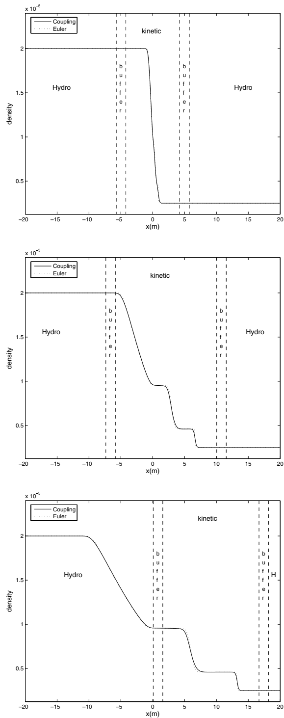
Fig. 12. Sod test 2: Density profile at different times t = 0.002 (top), t = 0.015 (middle), t = 0.03 (bottom). The solid line is the solution of the coupling model, the dotted line is that of the Euler system.
