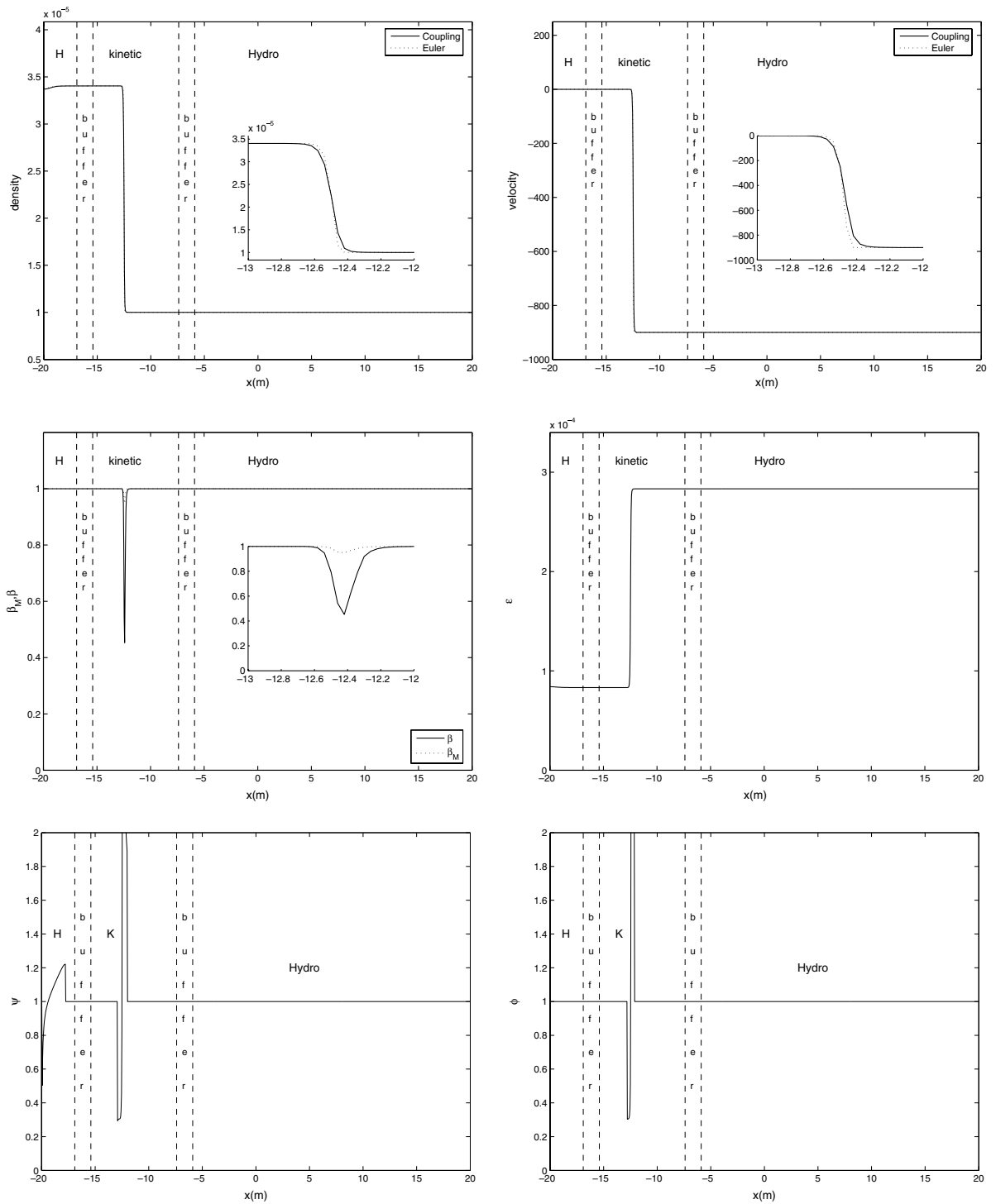
Fig. 7. Unsteady shock 2: Solution at t = 0.02 . Density (top left), velocity (top right), equilibrium fraction (middle left), Knudsen number (middle right), density smoothness indicator (bottom left), velocity smoothness indicator (bottom right). The small panels are a magnification of the solution close to the shock.
