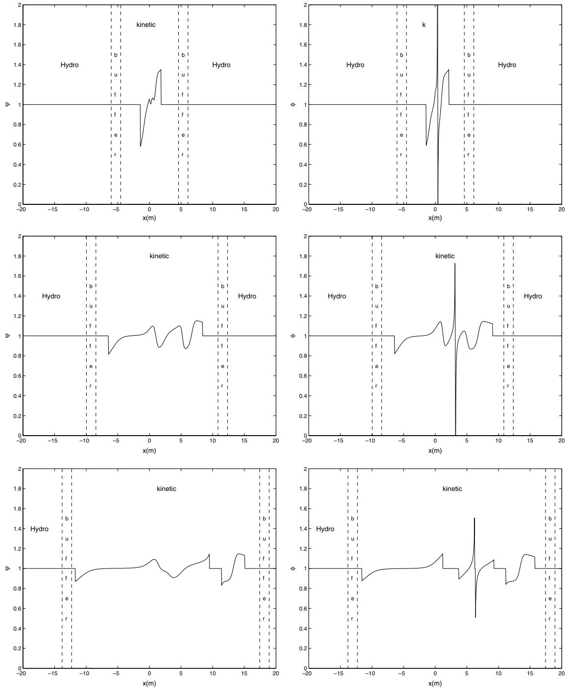
Fig. 11. Sod test I: Smoothness indicators for density (left) and velocity (right) at different times t = 0.002 (top), t = 0.015 (middle), t = 0.03 (bottom).
