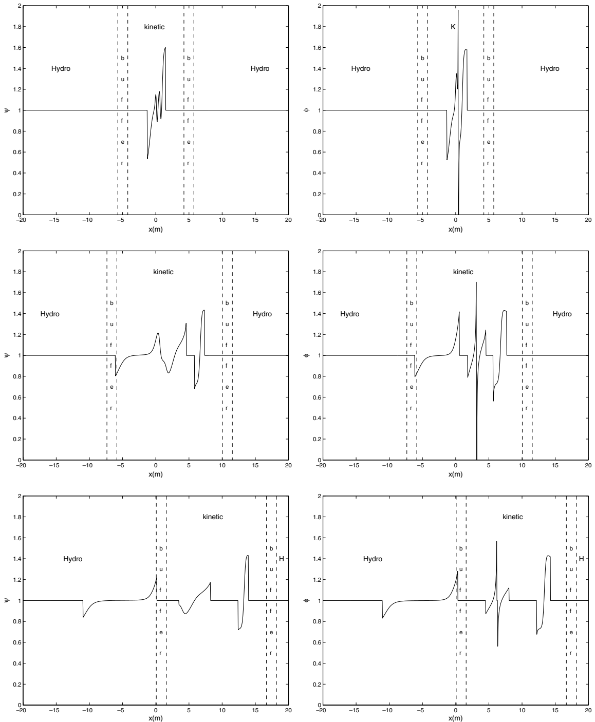
Fig. 15. Sod test 2: Smoothness indicators for density (left) and velocity (right) at different times t = 0.002 (top), t = 0.015 (middle), t = 0.03 (bottom).
