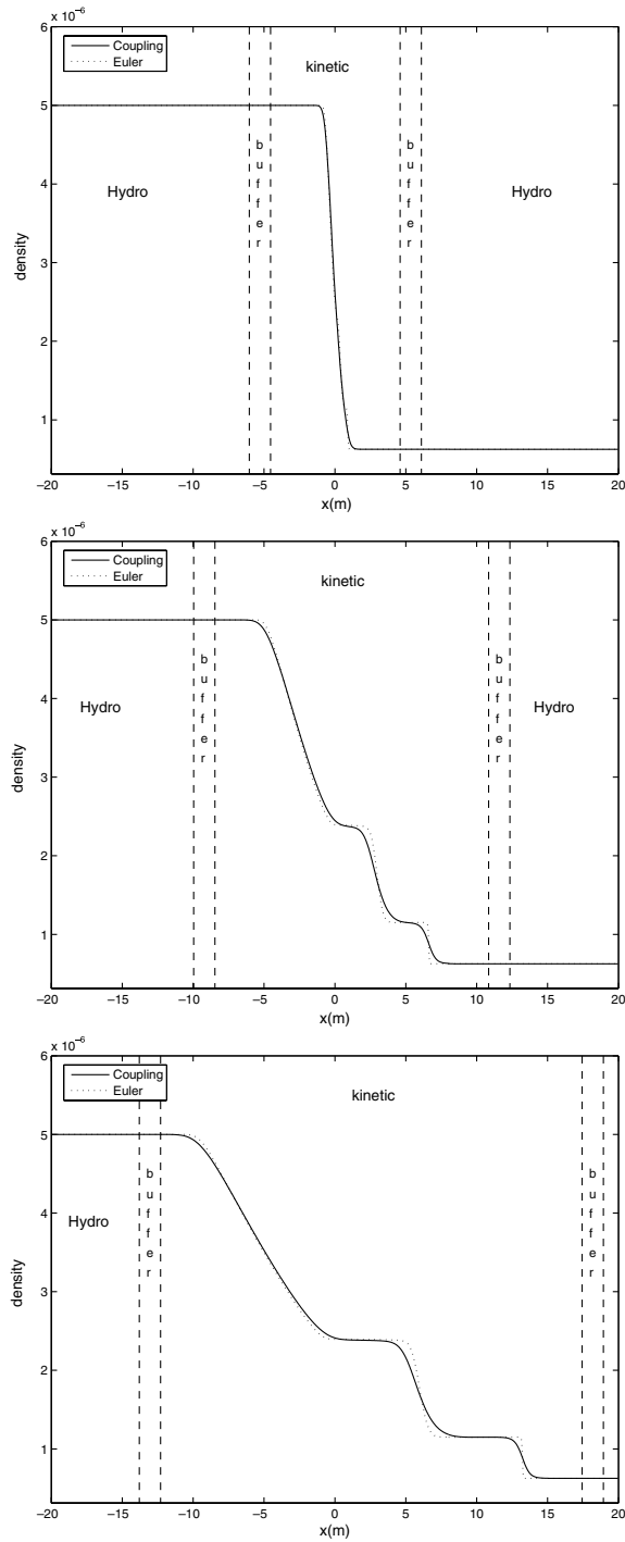
Fig. 8. Sod test 1: Density profile at different times t = 0.002 (top), t = 0.015 (middle), t = 0.03 (bottom). The solid line is the solution of the coupling model, the dotted line is that of the Euler system.
