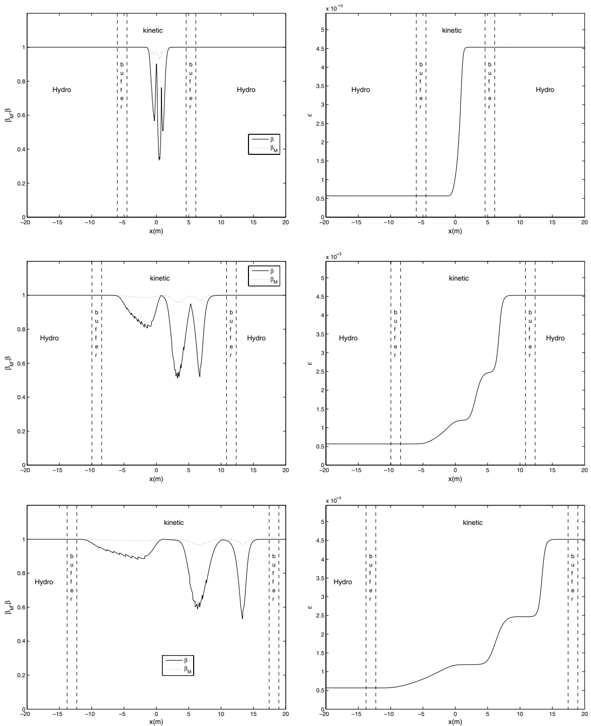
Fig. 10. Sod test 1: Equilibrium fraction profile (left), Knudsen number (right) at different times t = 0.002 (top), t = 0.015 (middle), t = 0.03 (bottom).
