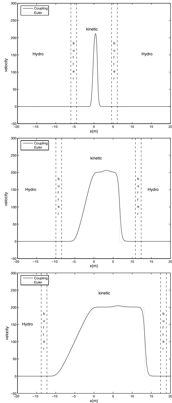
Fig. 9. Sod test 1: Velocity profile at different times t = 0.002 (top), t = 0.015 (middle), t = 0.03 (bottom). The solid line is the solution of the coupling model, the dotted line is that of the Euler system.
