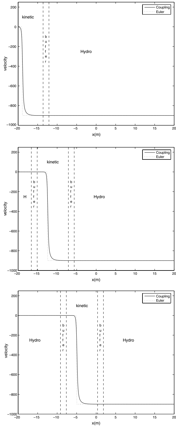
Fig. 3. Unsteady shock 1: Velocity profile at different times t = 0.002 (top), t = 0.02 (middle), t = 0.04 (bottom). The solid line is the solution of the coupling model, the dotted line is that of the Euler system.
