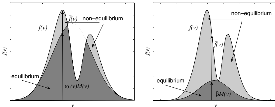
Fig. 1. Distribution function as a combination of equilibrium and non-equilibrium parts: representation (49) (left) and representation (51) (right).
