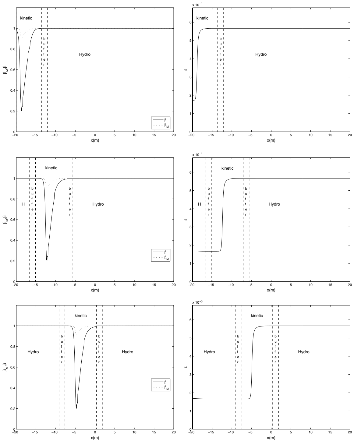
Fig. 4. Unsteady shock 1: Equilibrium fraction profile (left), Knudsen number (right) at different times t = 0.002 (top), t = 0.02 (middle), t = 0.04 (bottom).
