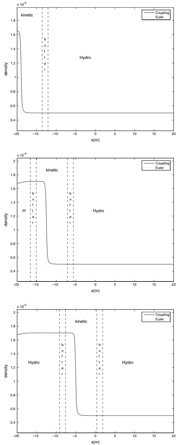
Fig. 2. Unsteady shock 1: Density profile at different times t = 0.002 (top), t = 0.02 (middle), t = 0.04 (bottom). The solid line is the solution of the coupling model, the dotted line is that of the Euler system.
